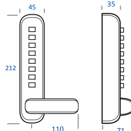
BL6000 SC Series Keypad
