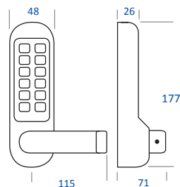
BL5400 SC Series Keypad
