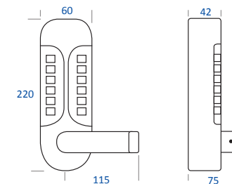
BL7000 SC Series Keypad
