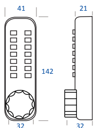
BL2500 SS Series Keypad
