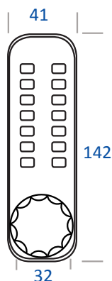
2500 Series Keypad
