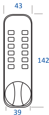
2900 Series Keypad
